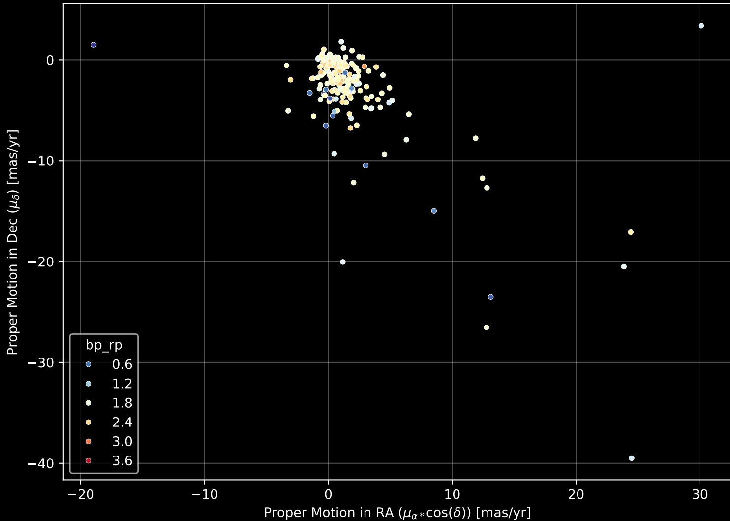
APOGEE DR17 Field: [169-04] Proper Motion Diagram (n= 195)
